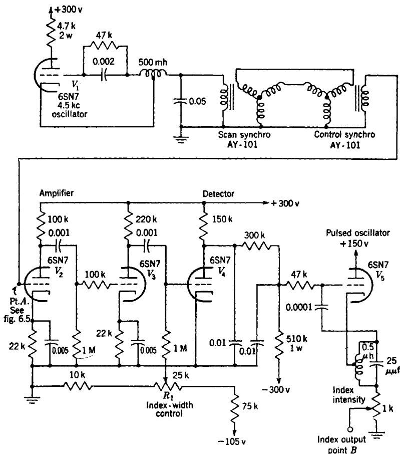
FIG. 6-4.—Synchro-null indices.
